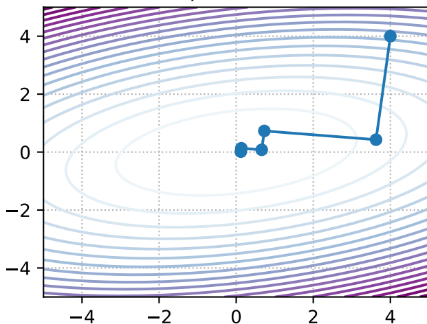
Steepest Descent
